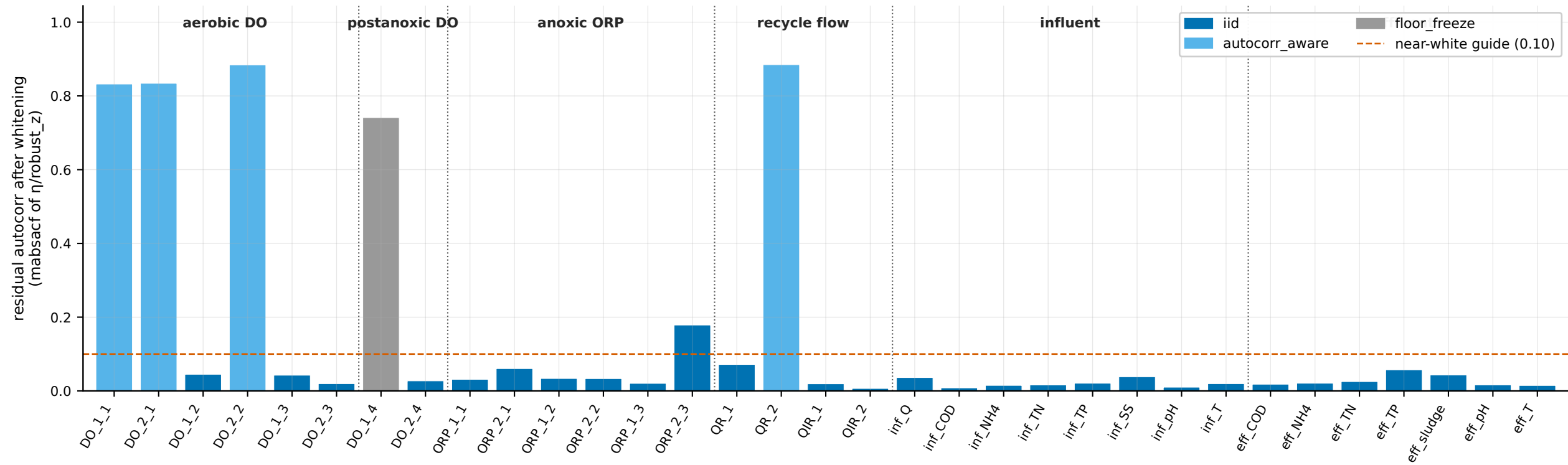
Figure 1.x Along-process whiteness gradient — clean innovations downstream, un-whitenable near-unit-root DO at the aerobic front (control/integrator fingerprint)
